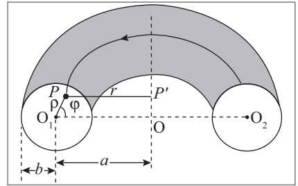
Figura 9.17 Bobina toroidal.
