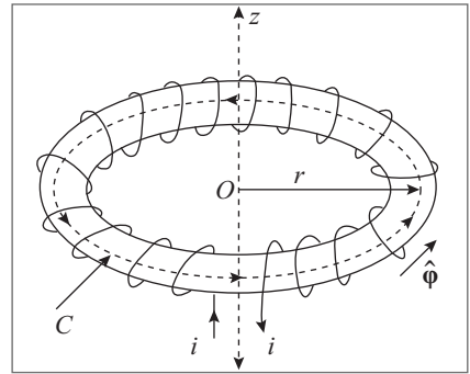
Figura 11.14 Anel de Rowland.
