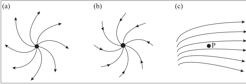
Figura 3.24 (a) \text{div } \mathbf{v}(P) > 0 (fonte); (b) \text{div } \mathbf{v}(P) < 0 (sorvedouro); (c) \text{div } \mathbf{v}(P) = 0 .
