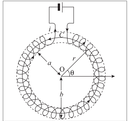
Figura 8.20 Bobina toroidal.
